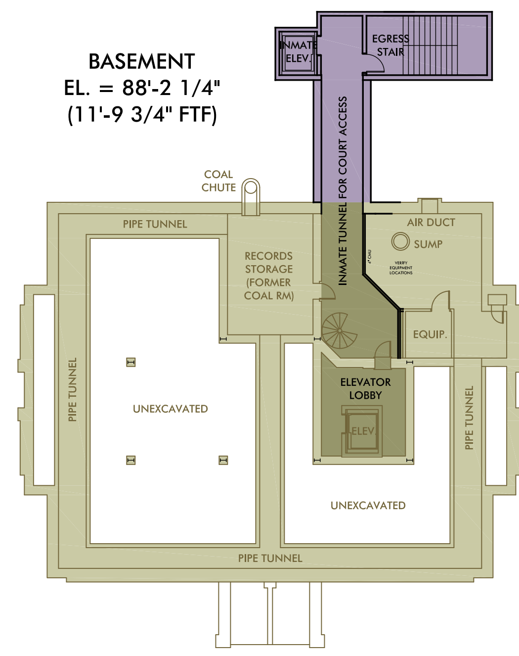
OPTION 5 BASEMENT TUNNEL PLAN SCALE: 1/16" = 1'-0"
